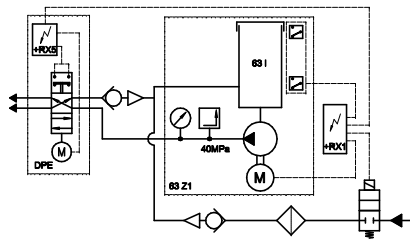
HYDRAULIC SCHEMA
